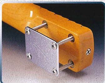
ANCHOR MOUNTED NECK JOINT
